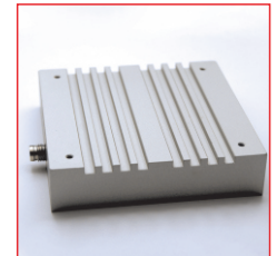
TOP-LIGHT-80 housing with integrated cooling ribs
